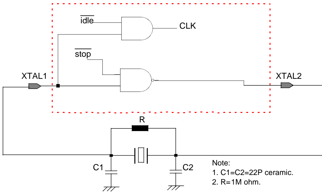
Fig.35 Oscillator Circuit.
